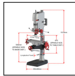
DCM 19 mm- Drilling... DRILLING CAPACITY 19 MM
